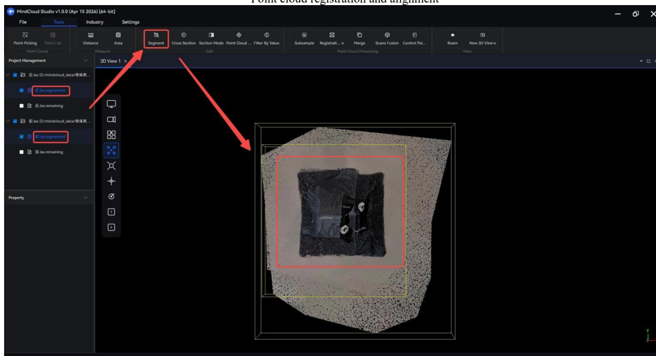
Crop stack
