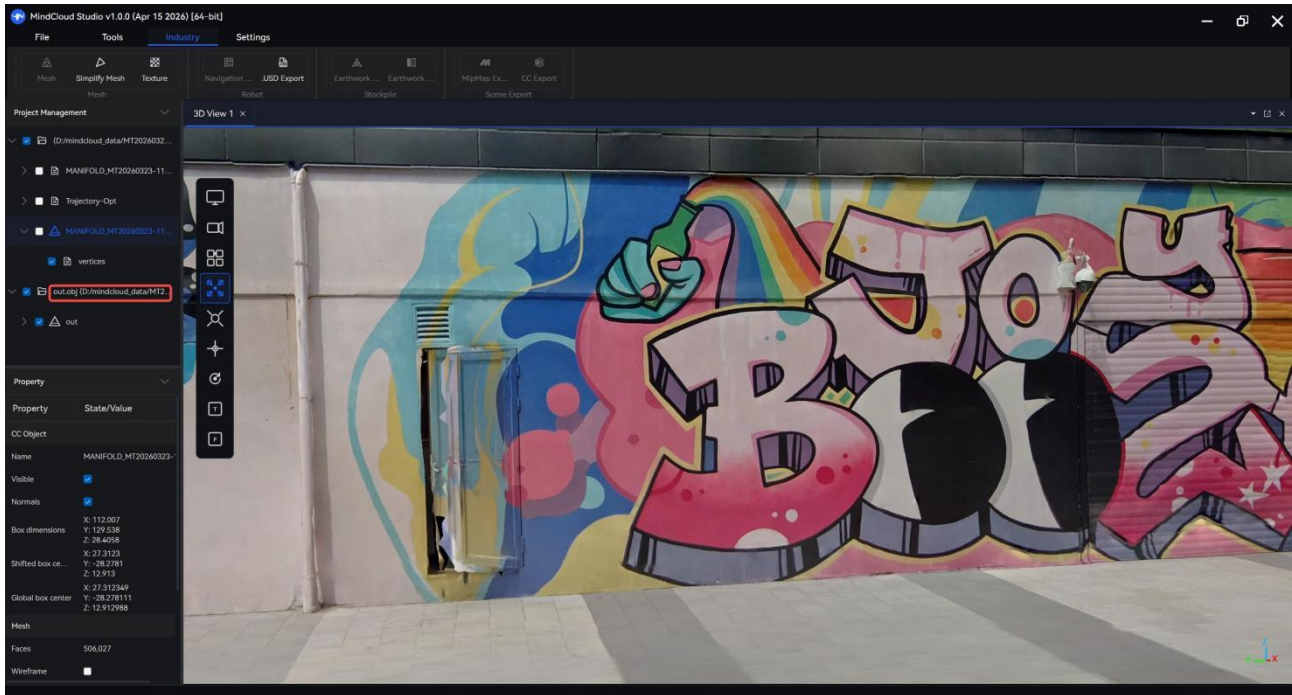
Mesh Model
