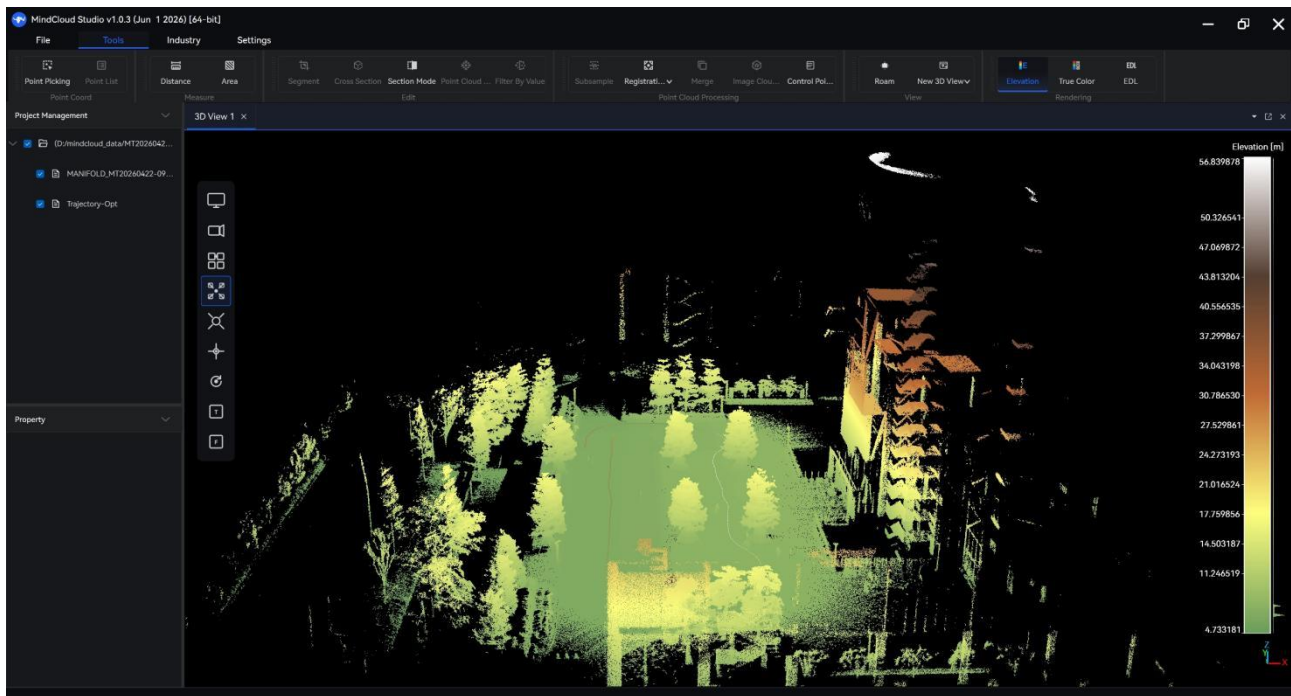
Elevation rendering
