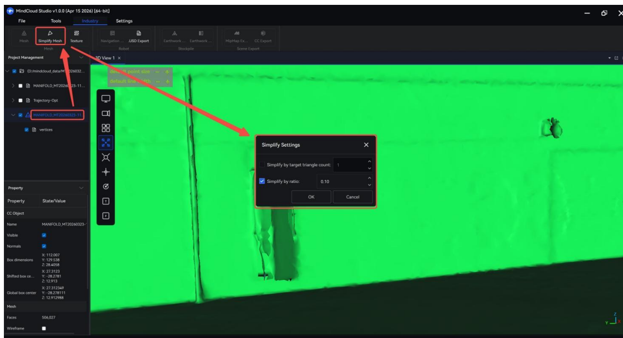
Grid Simplification
