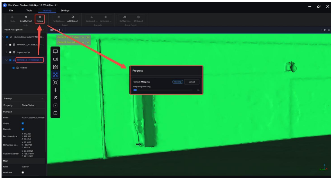
texture mapping
