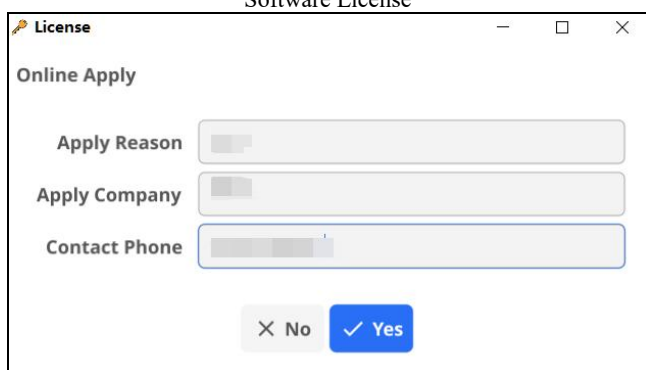
Network Authorization
