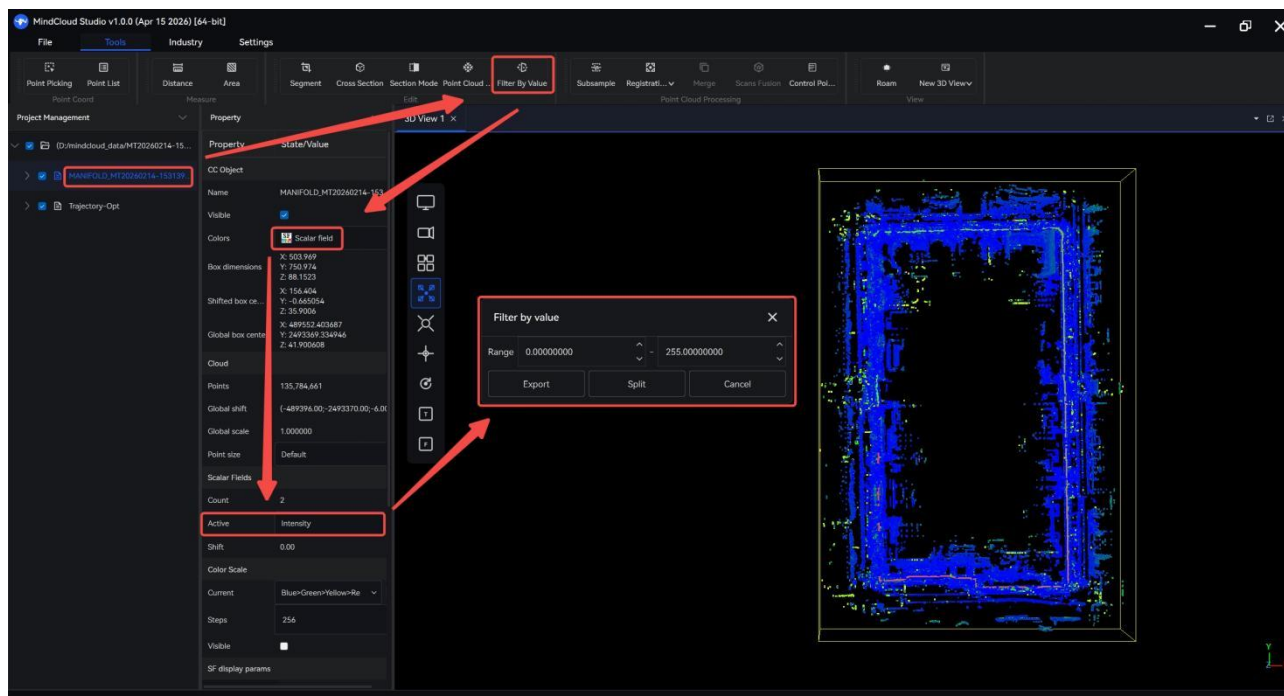
Intensity attribute
