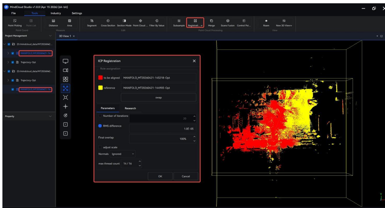
ICP
