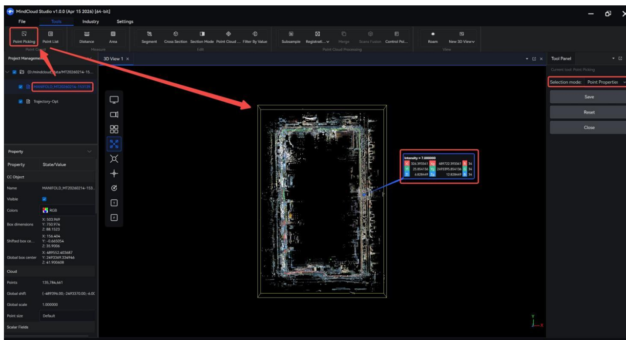
reconnaissance
