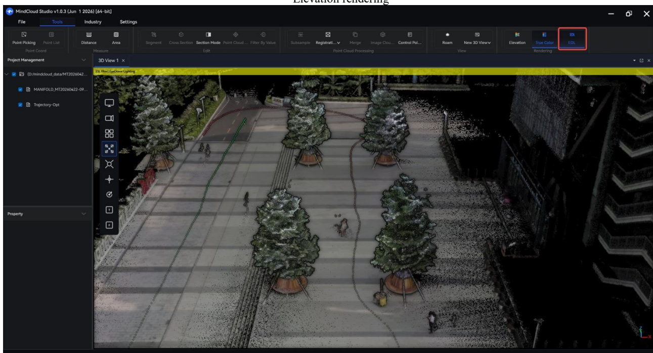
EDL rendering
