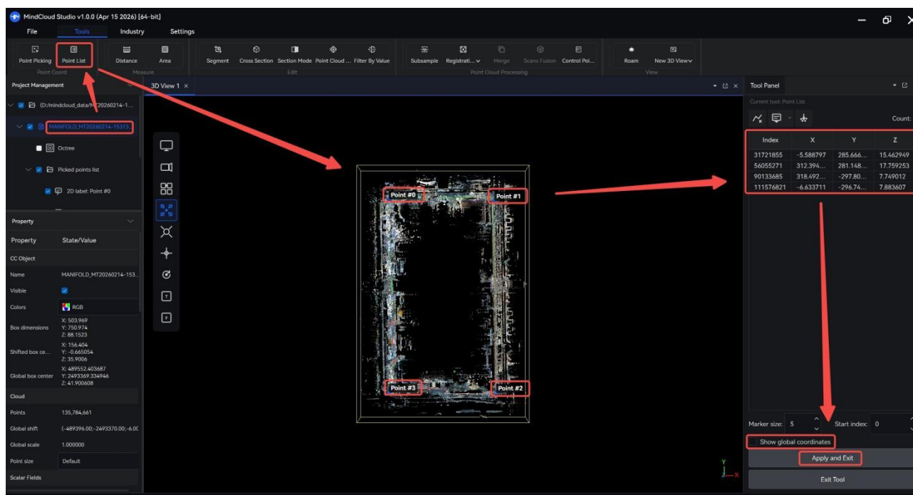
Point List
