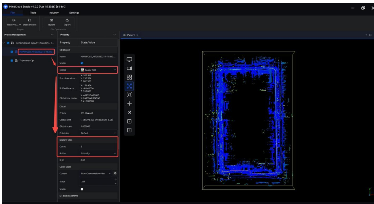
Scalar field
